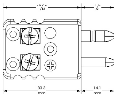
Plug Jab-In Ceramic 42C1XX00 Tubular Pins 42C4XX00 Solid Pins XX= Type Designator
